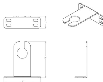
5000-GM-BZ Line Drawing
