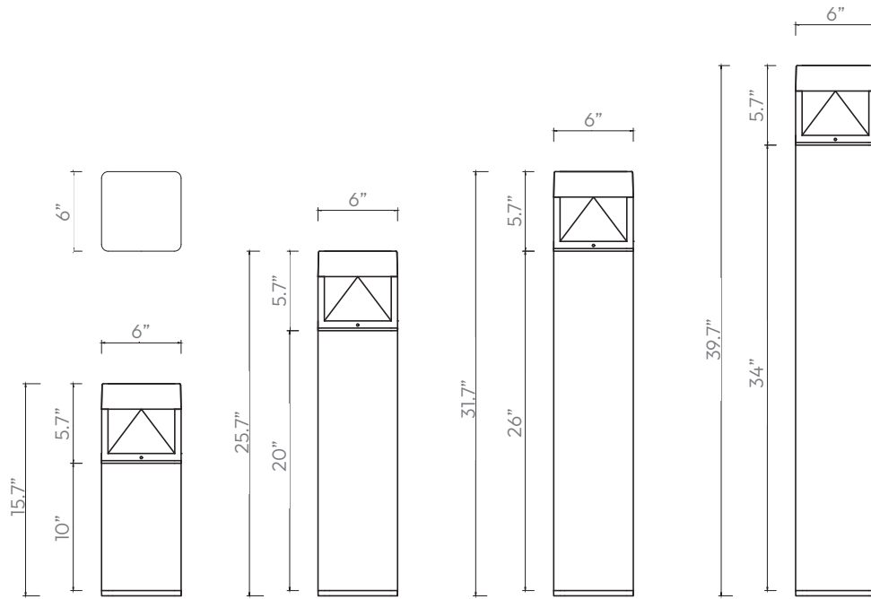
10" Shaft : 10"x 5.7"x 6" 20" Shaft: 20"x 5.7"x 6" 26" Shaft: 26"x 5.7"x 6" 34" Shaft: 34"x 5.7"x 6" (Sold Separately)
