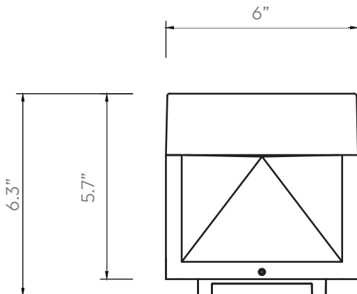
Technical Drawing: 5.7" (L) x 6" (W) x 6.3" (H)
