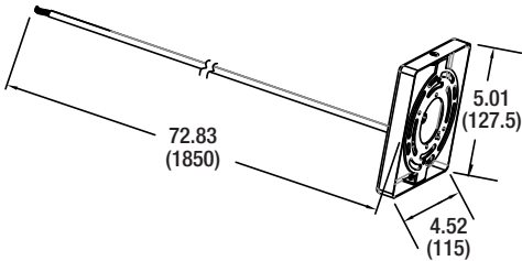
Suspension Kit with Canopy (62459 & 62461)
