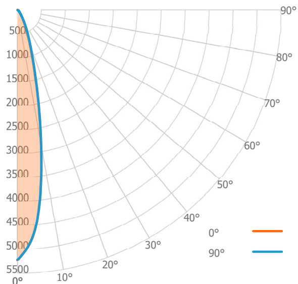
Candela Distribution
