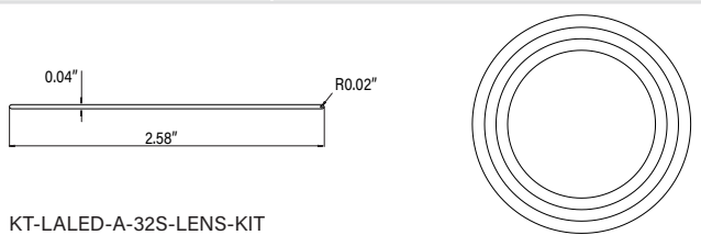
KT-LALED-A-32S-LENS-KIT
