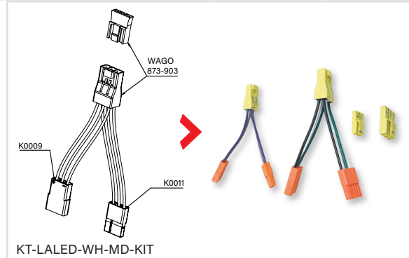
KT-LALED-WH-MD-KIT
