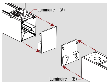
Step 1. Remove End Caps and open the top side of the fixture
