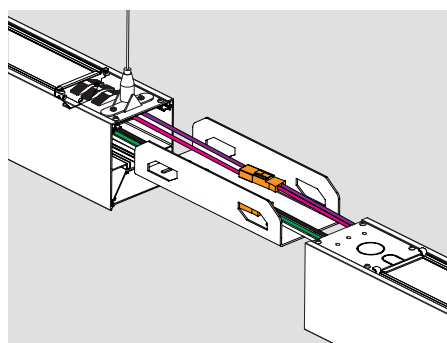
Step 2. Insert Linking Bracket, Connect wiring via included quick connects, Slide Fixture together, and fasten bracket with included buckles
