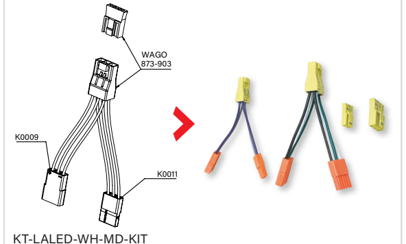
KT-LALED-WH-MD-KIT
