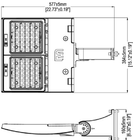
Flexible Arm
