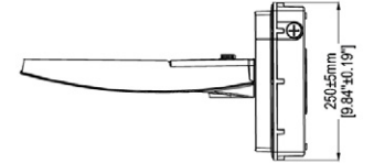
Fixed BBU Wall Mount
