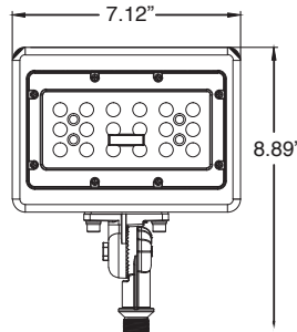
29W 1/2" Threaded Knuckle (Dedicated CCT)
