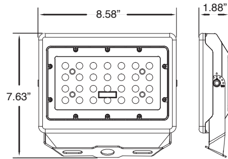
50W Yoke (Dedicated CCT)
