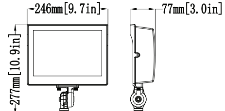
60W Threaded Knuckle (CCT Selectable)
