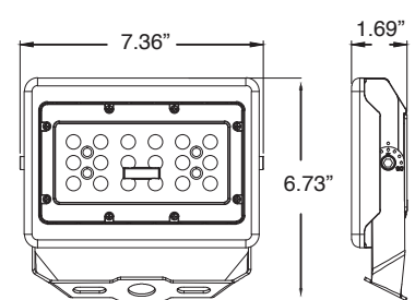
29W Yoke (Dedicated CCT)
