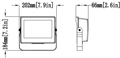
15-25W Yoke (CCT Selectable)
