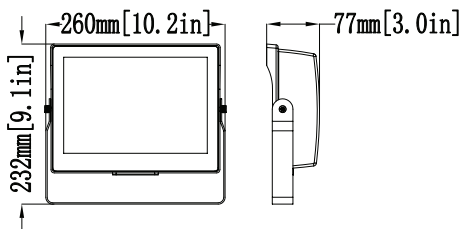
60W Yoke (CCT Selectable)
