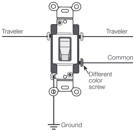
Traditional 3-way mechanical switch wiring
