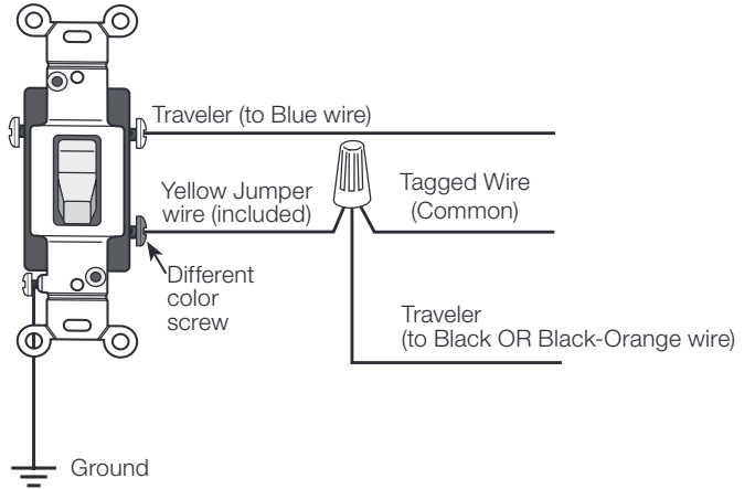
3-way mechanical switch wiring with dual tech sensor switch
