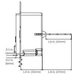
Voltage Barrier
