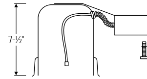
Ceiling Cut-out
