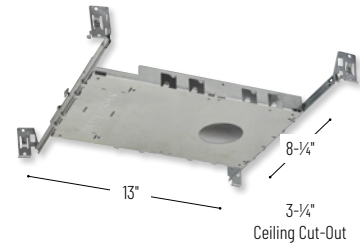
8-1/4" 3-1/4" Ceiling Cut-Out
