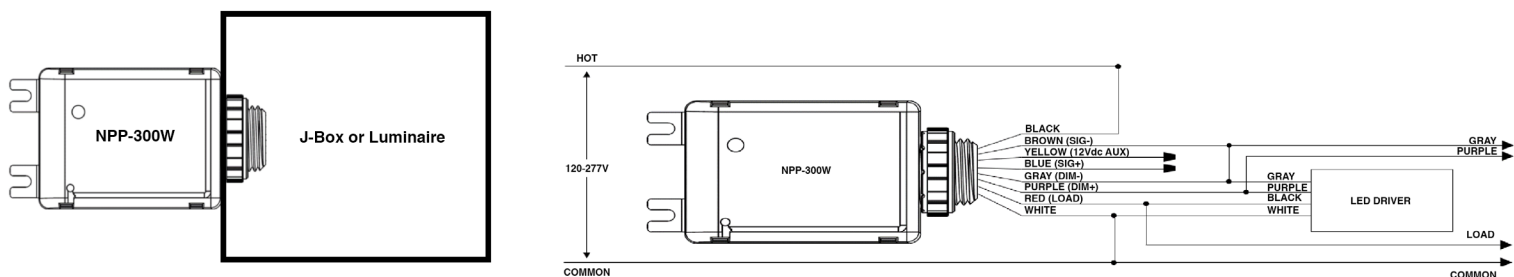
WIRING DIAGRAM WITHOUT NPPSL-PSW*
