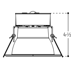
Ceiling Cut-Out: 4-3/4" Ø
