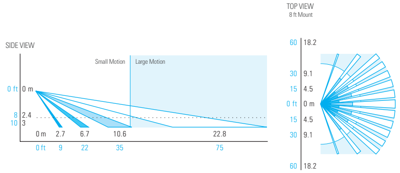
Diagram reflects sensor in first position. Adjust angle downward if mounting above 10 feet or to decrease gap directly under sensor.
