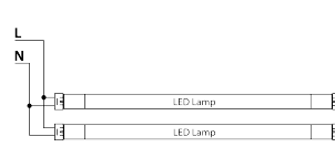
Single ended
