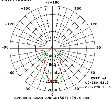
2ft Baffle Lens — Direct 20W / 5000K
