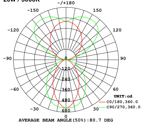
2ft Baffle Lens — Direct/Indirect 20W / 5000K
